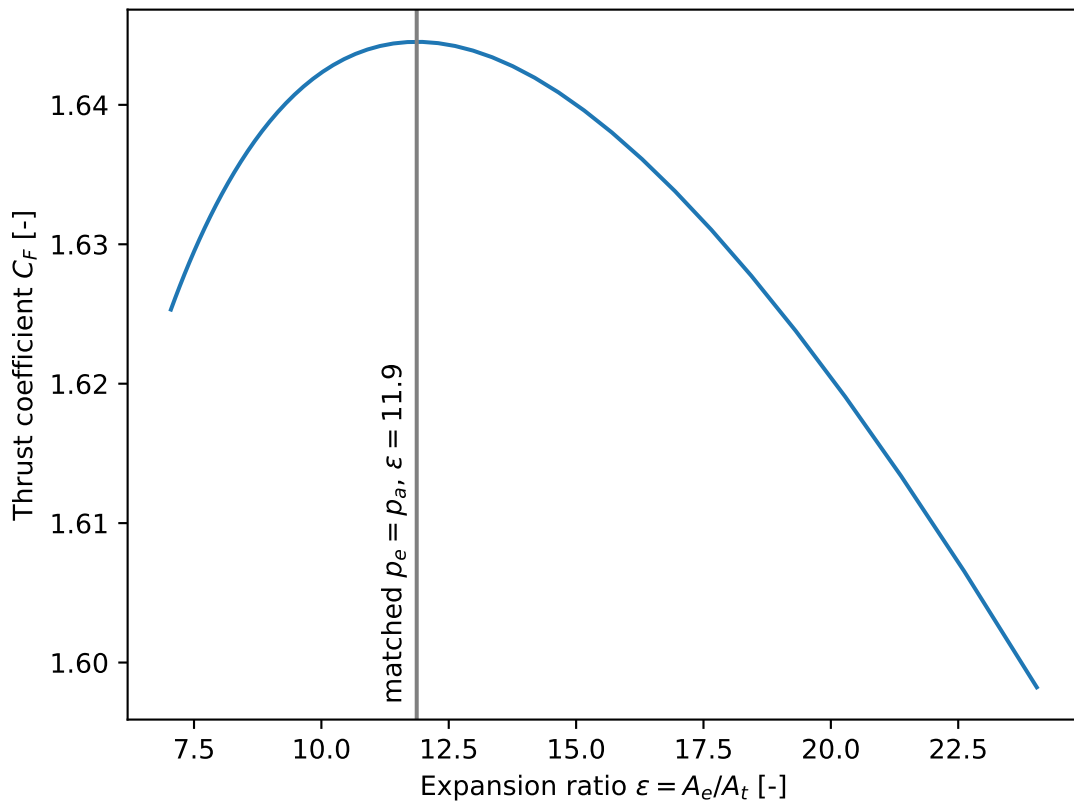
C_F vs expansion ratio at p_c = 10 MPa, p_a = 100 kPa
