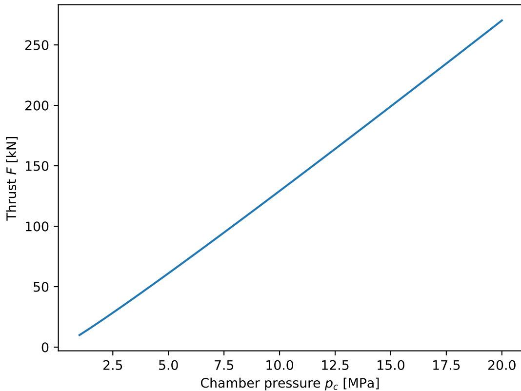
Thrust vs chamber pressure at p_e = p_a = 100 kPa
