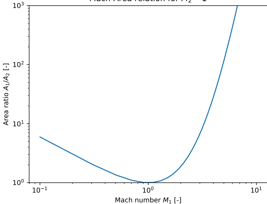
Mach-Area relation for M_2 = 1
