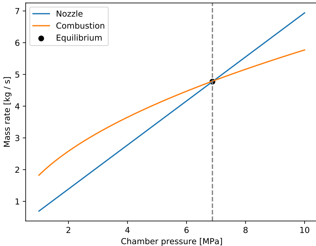
Chamber pressure: stable equilibrium, n = 0.5
